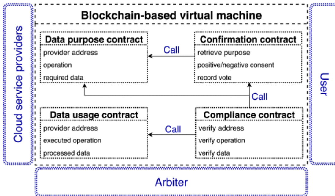
Figure 2. Proposed smart contracts.
